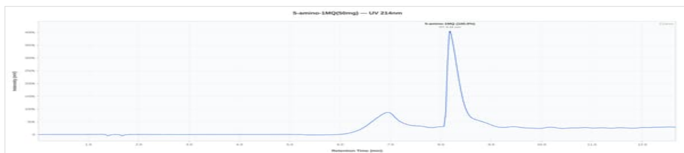
5 Amino 50mg - PS06-5AM50R: UV Chromatogram
